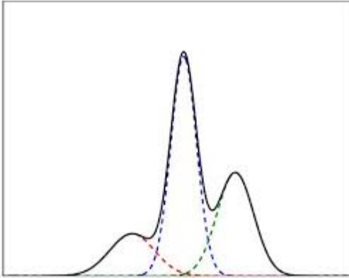
□ 1d model with K = 3 components
